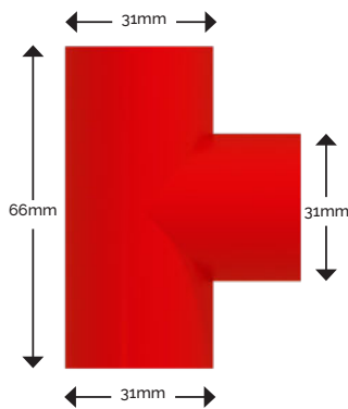
TEE ADAPTOR
