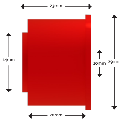
CAPILLARY ADAPTOR
