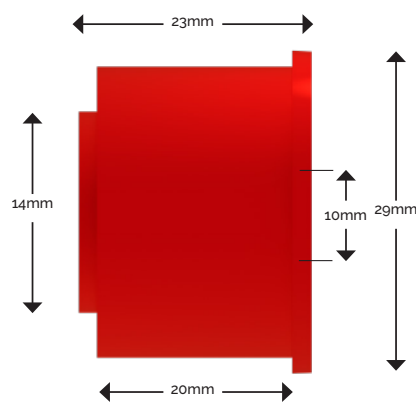
CAPILLARY ADAPTOR
